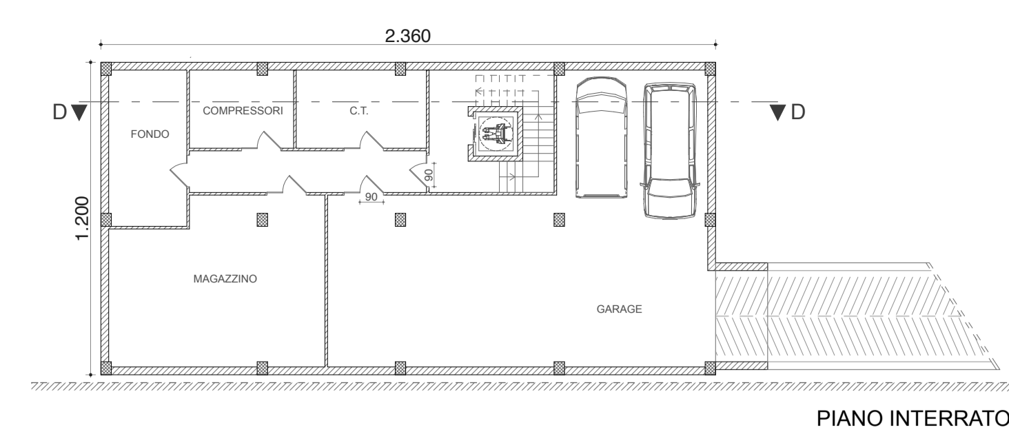
PIANO INTERRATO
